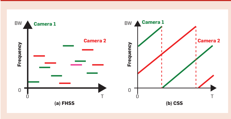
Figure 8. Distributed Interference Management approaches.
